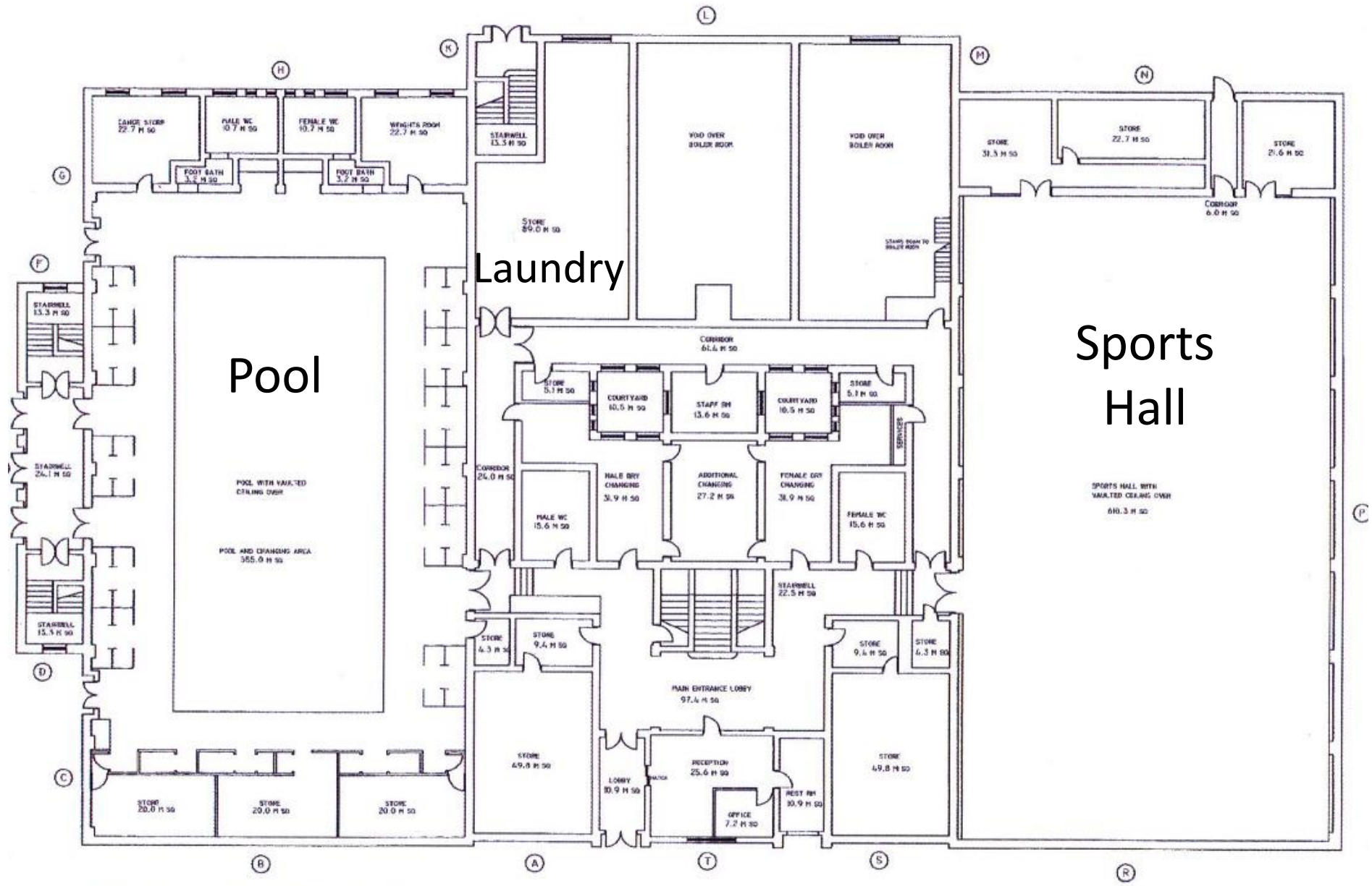
GROUND FLOOR PLAN 2537.0 M SQ
